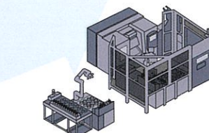
LB3000EX III + smarTwinCELL + AGV
